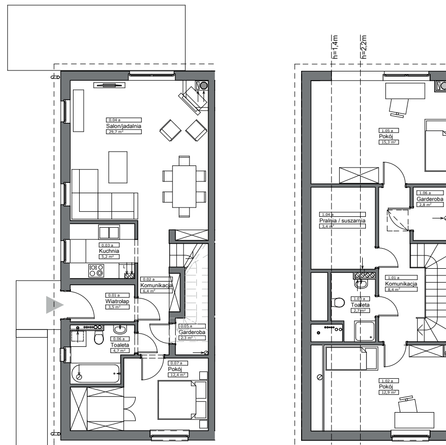
PARTER
